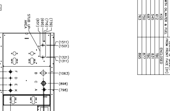
TANKBASE PLAN SHOWING MOUNTING POINTS
