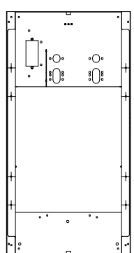
GROUND FIXING LOCATIONS - VIEW FROM BOTTOM
