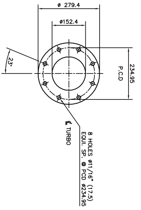
EXHAUST OUTLET DETAILS SCALE 2.5:1
